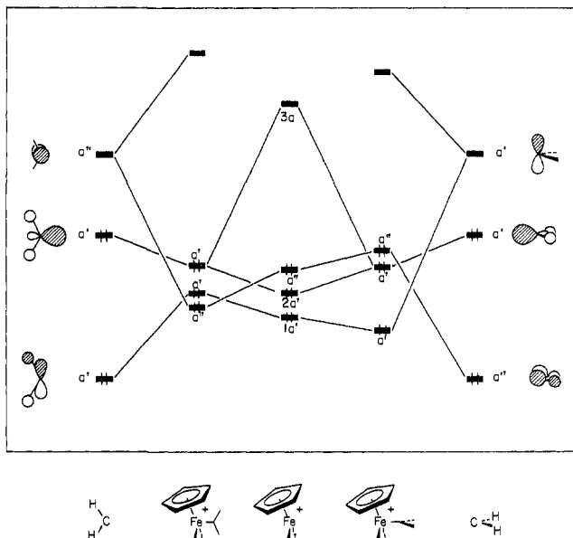
Figure 3. Orbital interaction diagram for \text{CpFe}(\text{CO})_2^+ and a carbene in two different orientations, 12 and 13 .
