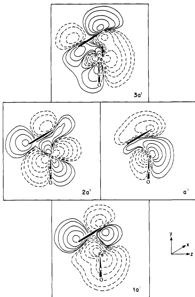
Figure 2. A plot of the four valence orbitals of a \text{CpFe}(\text{CO})_2^+ fragment. The contour levels of \psi are 0.2, 0.1, 0.55, 0.025, 0.01, and 0.005. The symmetric orbitals are plotted in the yz plane, the antisymmetric orbitals in a plane parallel and 0.2 Å from the yz plane.
